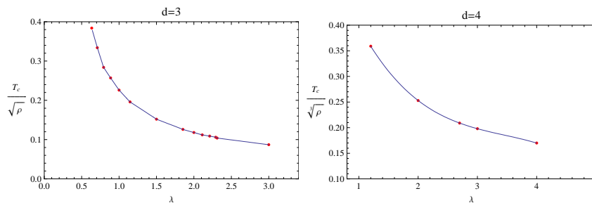
Figure 3. The dependence of the critical temperature on the dimensions of the dual condensates in 2 + 1 and 3 + 1 boundary theories
