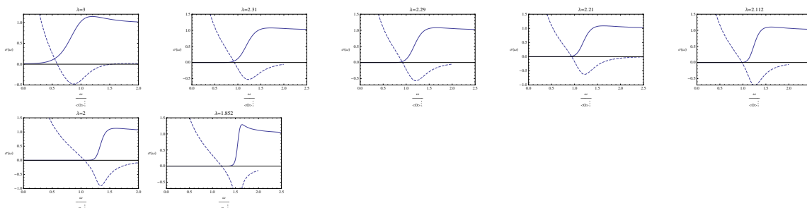
Figure 14. Plots of the frequency dependent conductivity for condensates of class \Psi_{\lambda_+} . The frequency is normalized by the condensate. The plots are labelled by the dimension of the operator in the boundary theory
