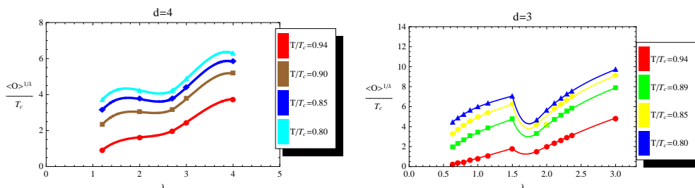
Figure 2. The amount of condensates as a function of the dimension of the dual operator (right) computed at different fixed temperatures. The dots represent the actual value and the continuous line is an interpolation between the actual values. This form of representation is used in the rest of the report.
