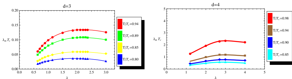
Figure 11. Magnetic penetration depth as a function \lambda .
