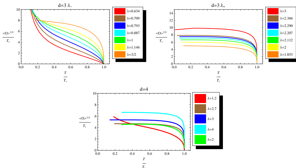
Figure 1. The condensates as a function of temperature for various condensates \mathcal{O}_\lambda in the boundary theory. The figures are labelled by the scaling dimensions of the dual condensates. The upper left graphs are condensates dual to the modes of the scalar field with slower fall-off \Psi_{\lambda_-} , while the upper right figure shows the condensates dual to the modes of scalar fields with faster fall-off \Psi_{\lambda_+} . The graphs are labelled by \lambda_- and \lambda_+ to distinguish between the two classes of condensates in the 2 + 1 boundary theory. Below the two graphs is the condensates as a function of temperature for various condensate \mathcal{O}_\lambda in 3 + 1 dual field theory
