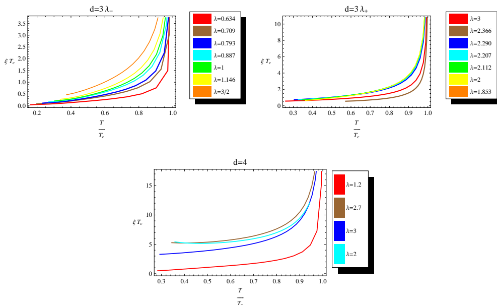
Figure 8. Superconducting coherence length of holographic superconductors plotted as a function of temperature.
