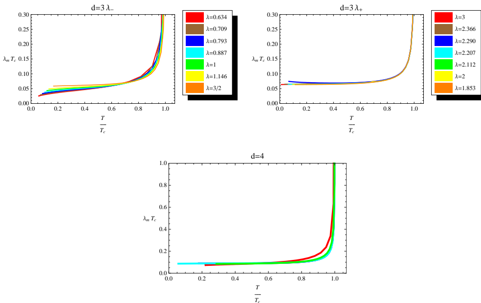
Figure 6. The magnetic penetration depth below the critical temperature in the dual field theory.
