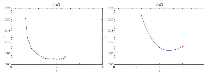
Figure 12. Ginzburg-Landau parameter against \lambda .
