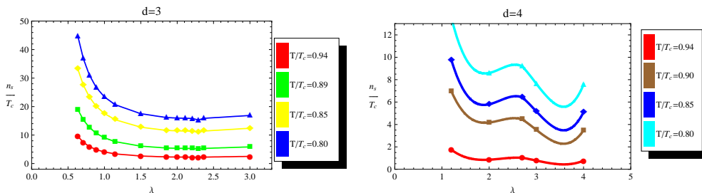
Figure 5. Superfluid density as function of the dimension of the dual operator, at different fixed temperatures
