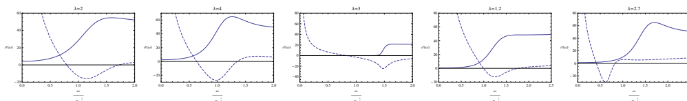
Figure 15. Plots of the conductivity versus the frequency normalized by the condensate in the 3 + 1 boundary theory. Each of the plots was calculated at T/T_c = 0.3 and they are labelled by the dimension of the dual condensates.
