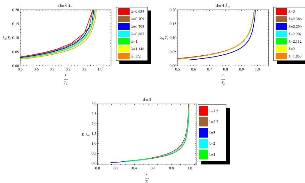
Figure 10. Magnetic penetration depth below the critical temperature in the superconducting phase.
