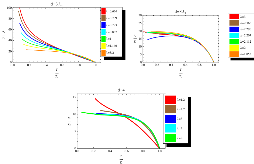
Figure 4. Superfluid density below the critical temperature in the boundary theory.
