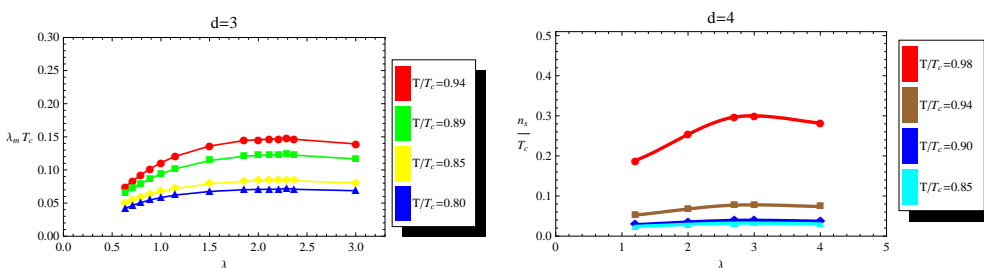
Figure 7. Magnetic penetration depth as function of the dimension of the dual operator, at temperatures below T_c .
